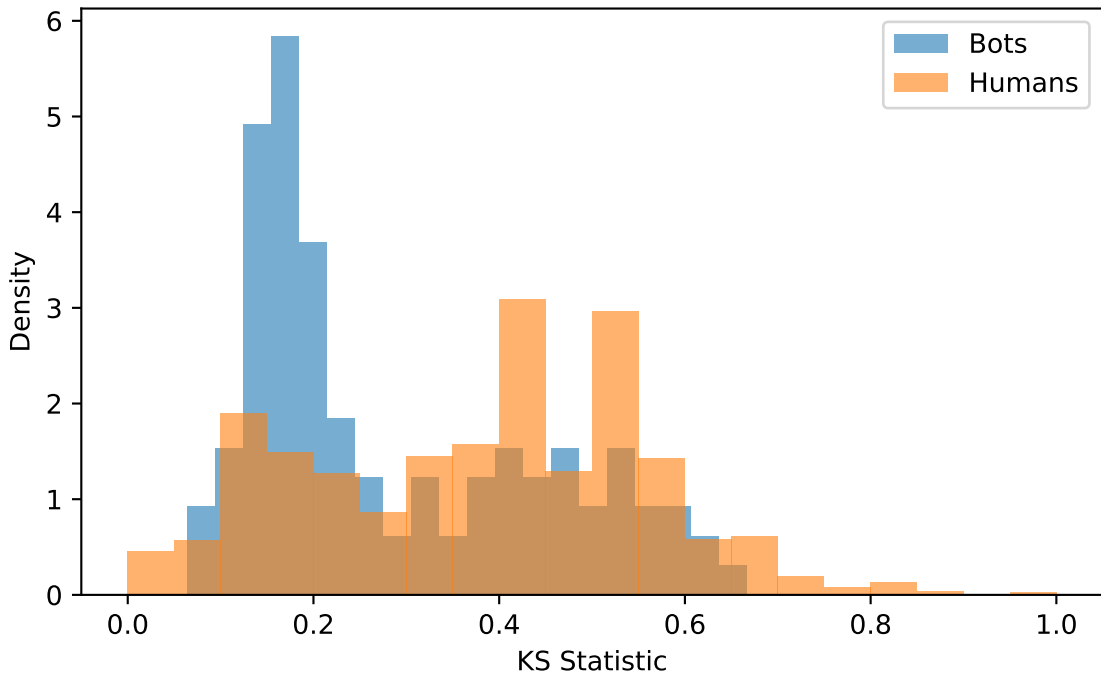
KS Test: Ks Lognormal
