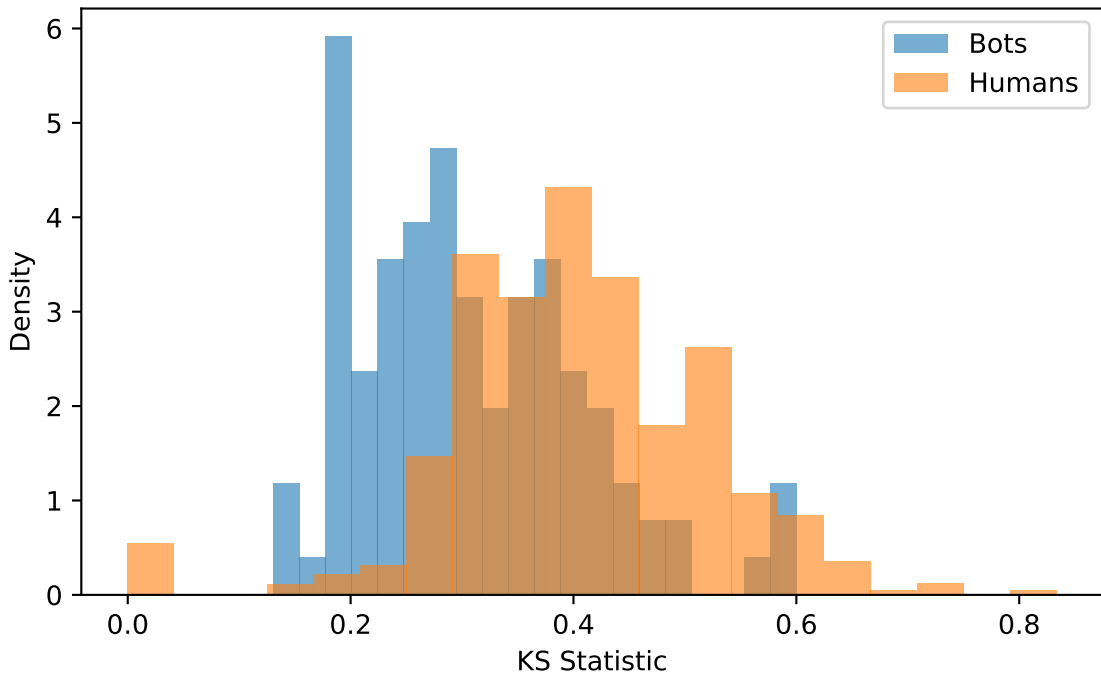
KS Test: Ks Normal
