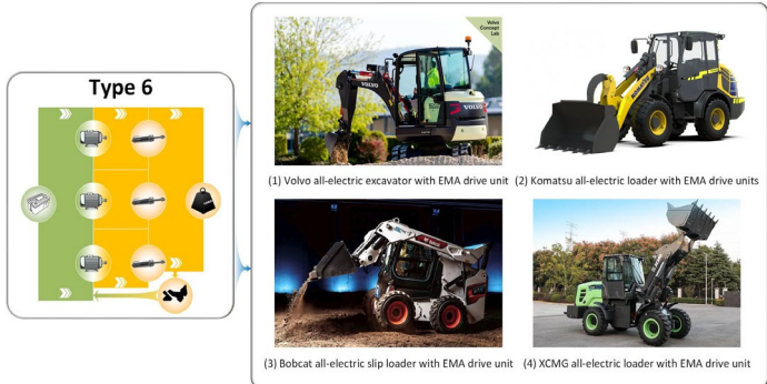
Fig. 20 P-ECM with a “distributed power and distributed electromechanical control system” configuration (Cited from [Volvo Construction Equipment; Moog Inc; Bobcat Company; XCMG Group, 2025])
