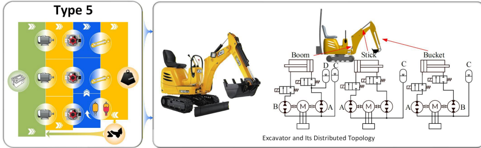
Fig. 14 Excavator system architecture (2) with distributed power and distributed volumetric control system (Cited from [Zhang et al., 2017a]).
