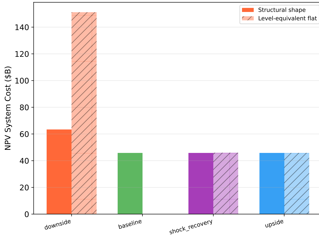
Ndc3 Unconditional
