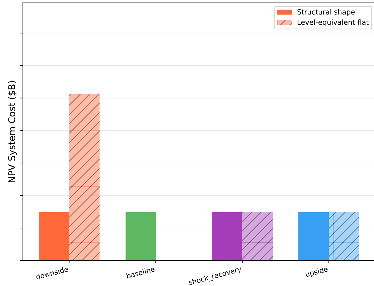
Ndc3 Conditional
