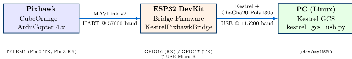
Figure 1: System Communication Topology: Pixhawk CubeOrange+ \rightarrow ESP32 Bridge \rightarrow PC Kestrel GCS
