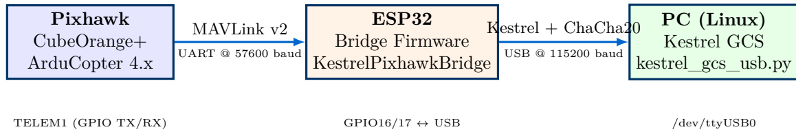
Figure 1: System Communication Topology: Pixhawk → ESP32 Bridge → PC GCS
