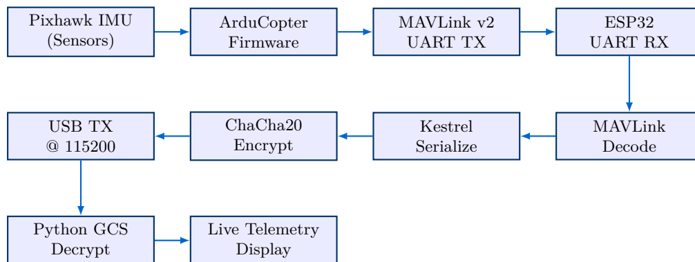
Figure 2: End-to-End Data Flow: Pixhawk IMU to GCS Display
