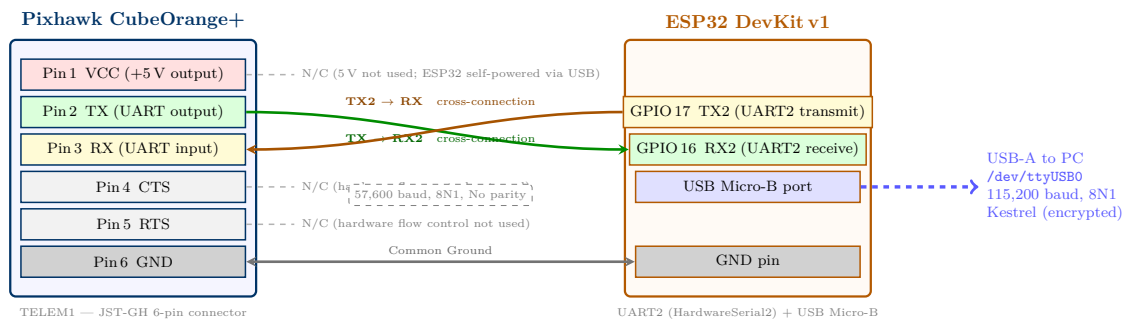
Figure 1: Physical Pin Wiring: Pixhawk CubeOrange+ TELEM1 (JST-GH 6-pin) to ESP32 DevKit v1 UART2 GPIO. Signal wires are cross-connected (TX ↔ RX). Pins 1, 4, and 5 are left unconnected (N/C).
