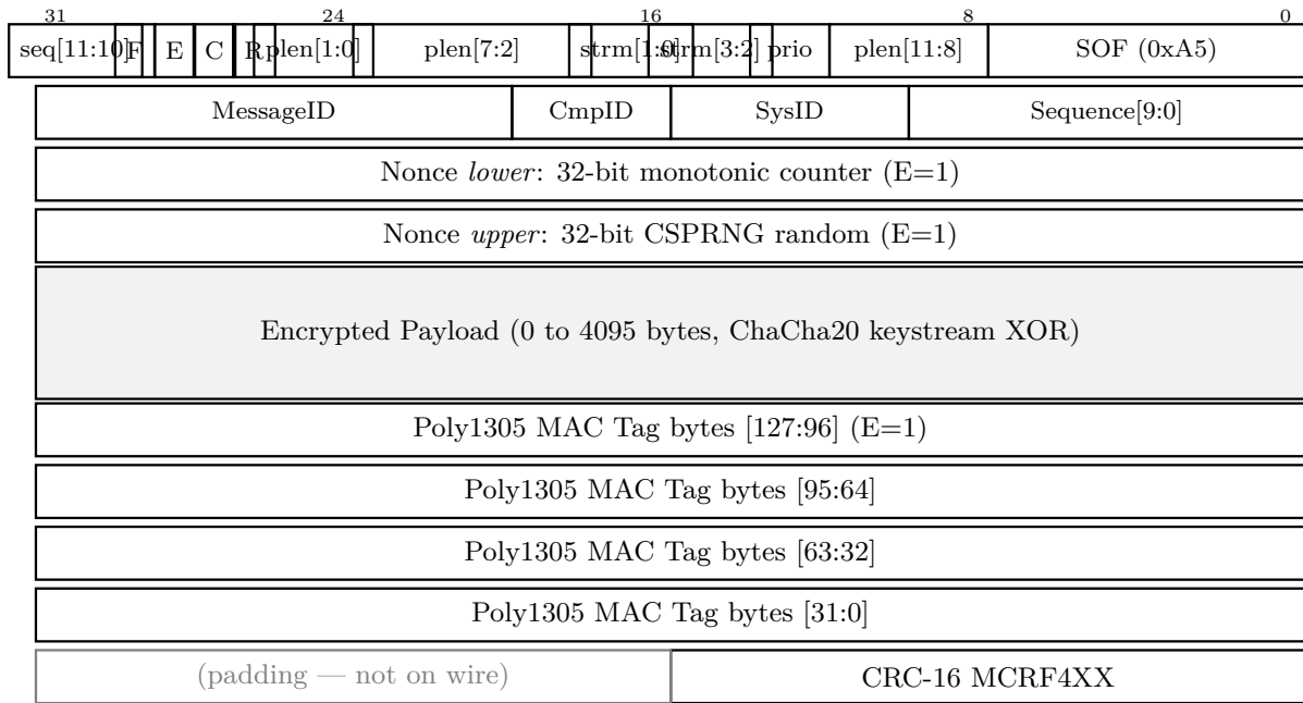
Figure 4: Kestrel Core Packet Wire Format (encrypted, unfragmented variant). R = Reserved(0); C = KS_FLAG_COMPRESSED (LZ4); E = KS_FLAG_ENCRYPTED (ChaCha20-Poly1305); F = KS_FLAG_FRAGMENTED. Fields plen , seq , and strm are split across bytes per the Kestrel Core Spec Section 3.1.
