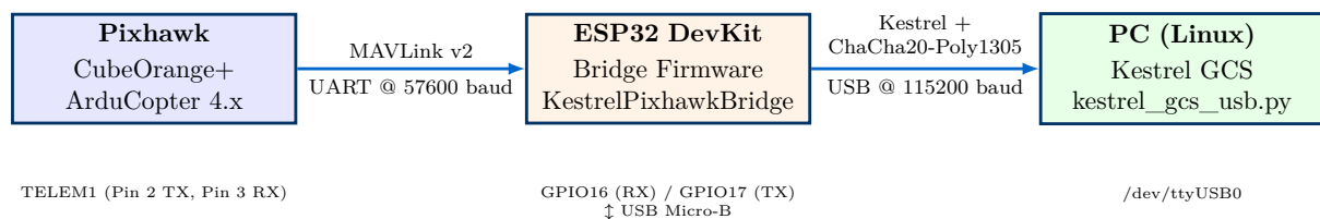
Figure 2: System Communication Topology: Pixhawk CubeOrange+ → ESP32 Bridge → PC Kestrel GCS
