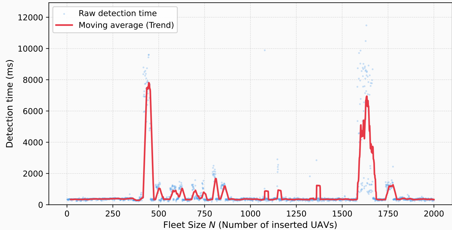
Conflict Detection Time Growth — Empirical O(\log N) Validation
