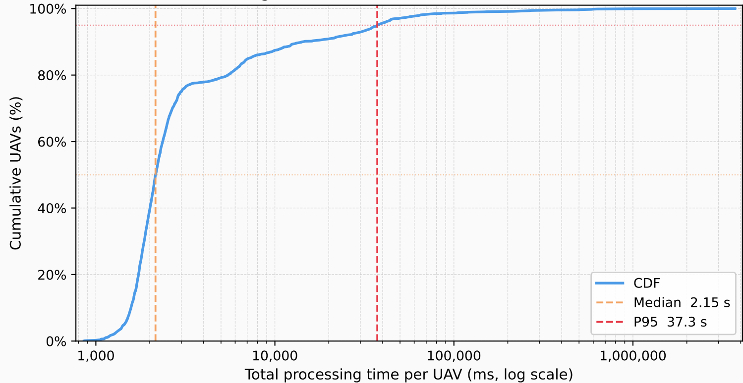
Total Processing Time CDF — Incremental Benchmark (2 000 UAVs)
