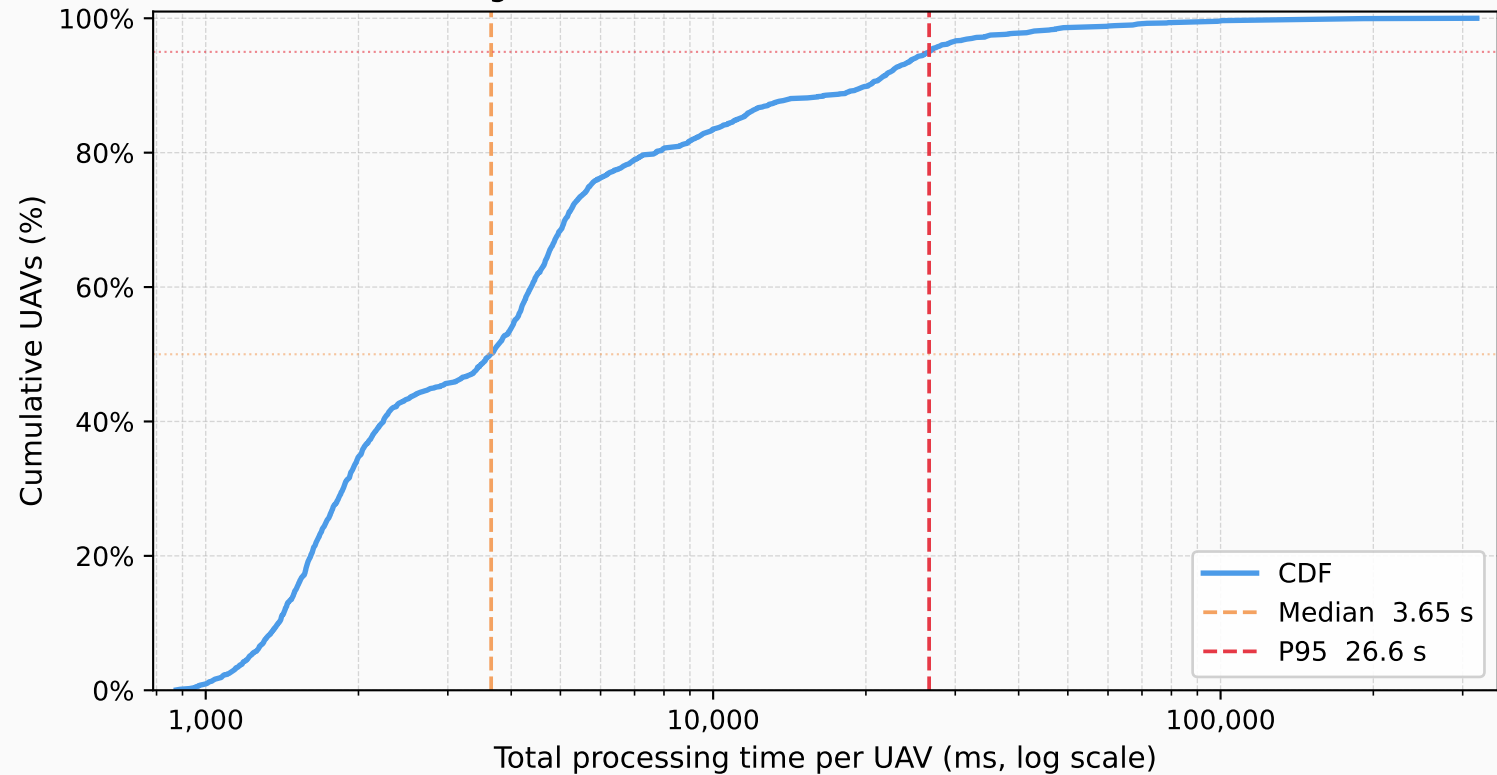
Total Processing Time CDF — Incremental Benchmark Fast (2 000 UAVs)
