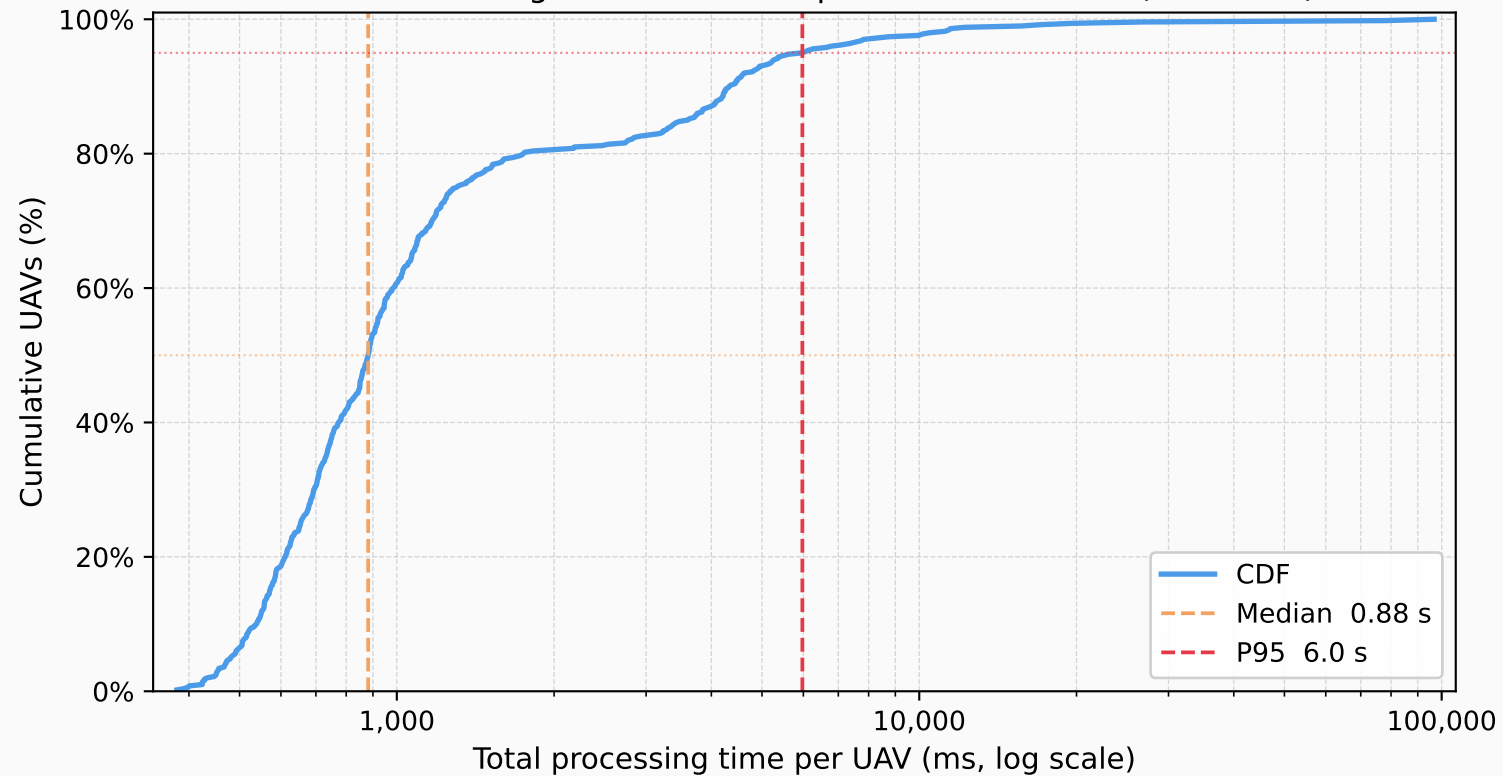
Total Processing Time CDF — Sequential Benchmark (500 UAVs)
