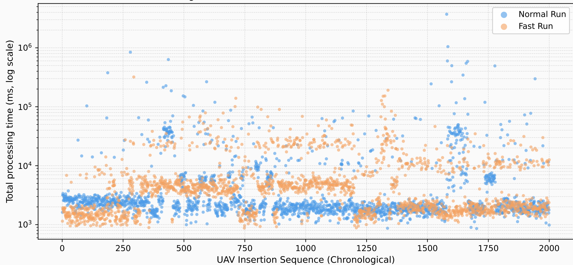
Processing Time Evolution — Incremental Benchmark (2 000 UAVs)
