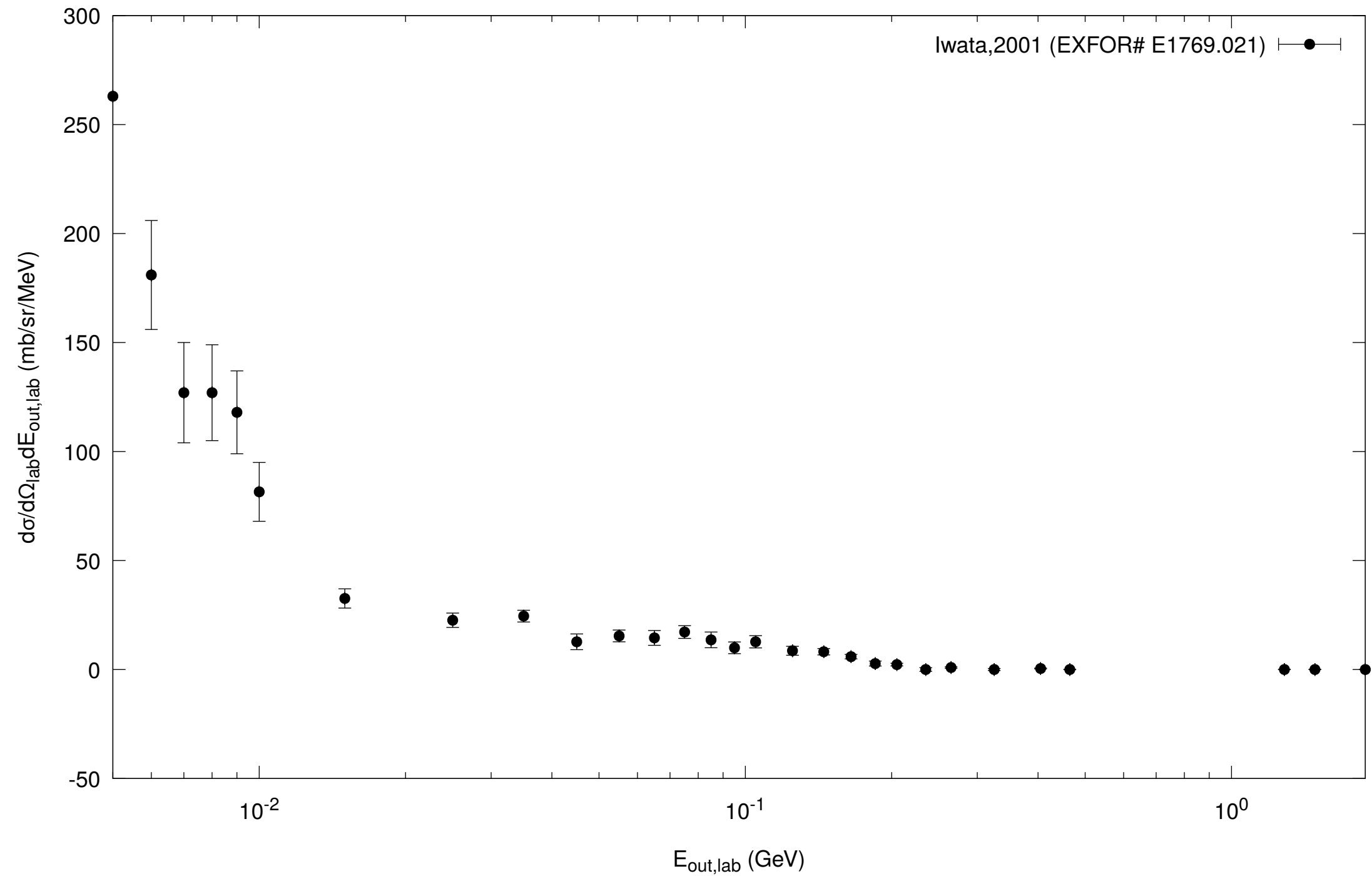
Pb( ^{12}\text{C}, n+x ), E_{\text{inc}}=3.48 GeV, \theta_{\text{lab}}=60 deg
