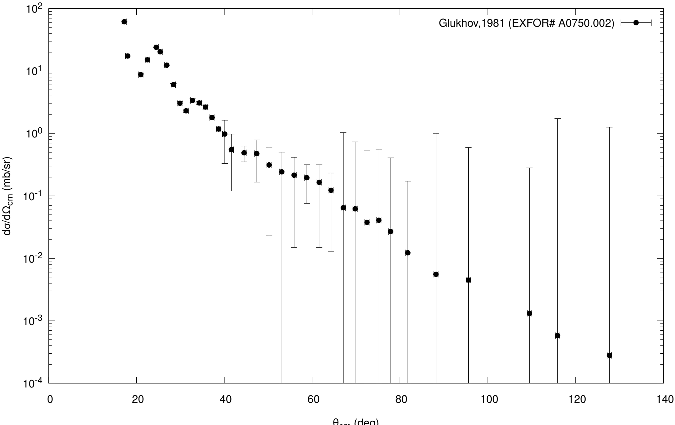
^{12}\text{C}(^6\text{Li}, \text{el})^{12}\text{C} , E_{\text{inc}}=90 \text{ MeV}
