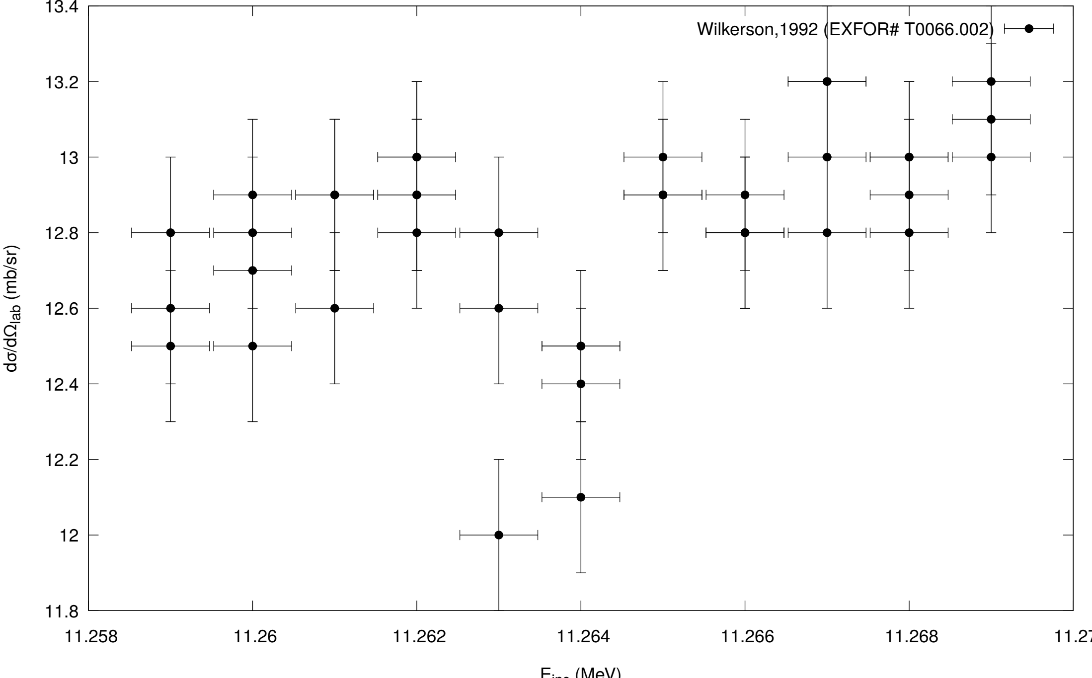
^{16}\text{O}(\text{p},\text{el})^{16}\text{O} , \theta_{\text{lab}}=142^\circ
