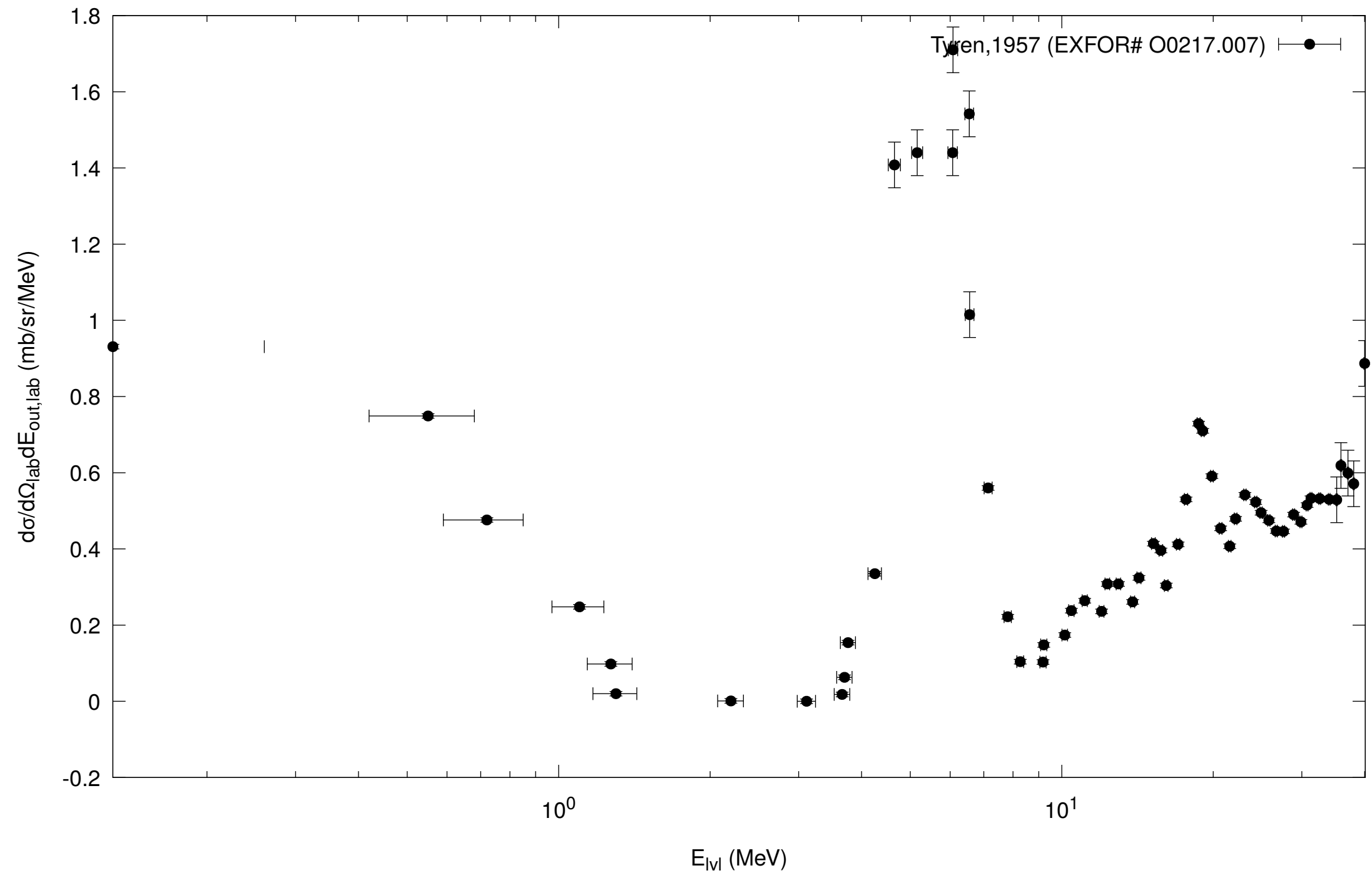
^{16}\text{O}(\text{p, inl})^{16}\text{O} , E_{\text{inc}}=181 MeV, \theta_{\text{lab}}=30 deg
