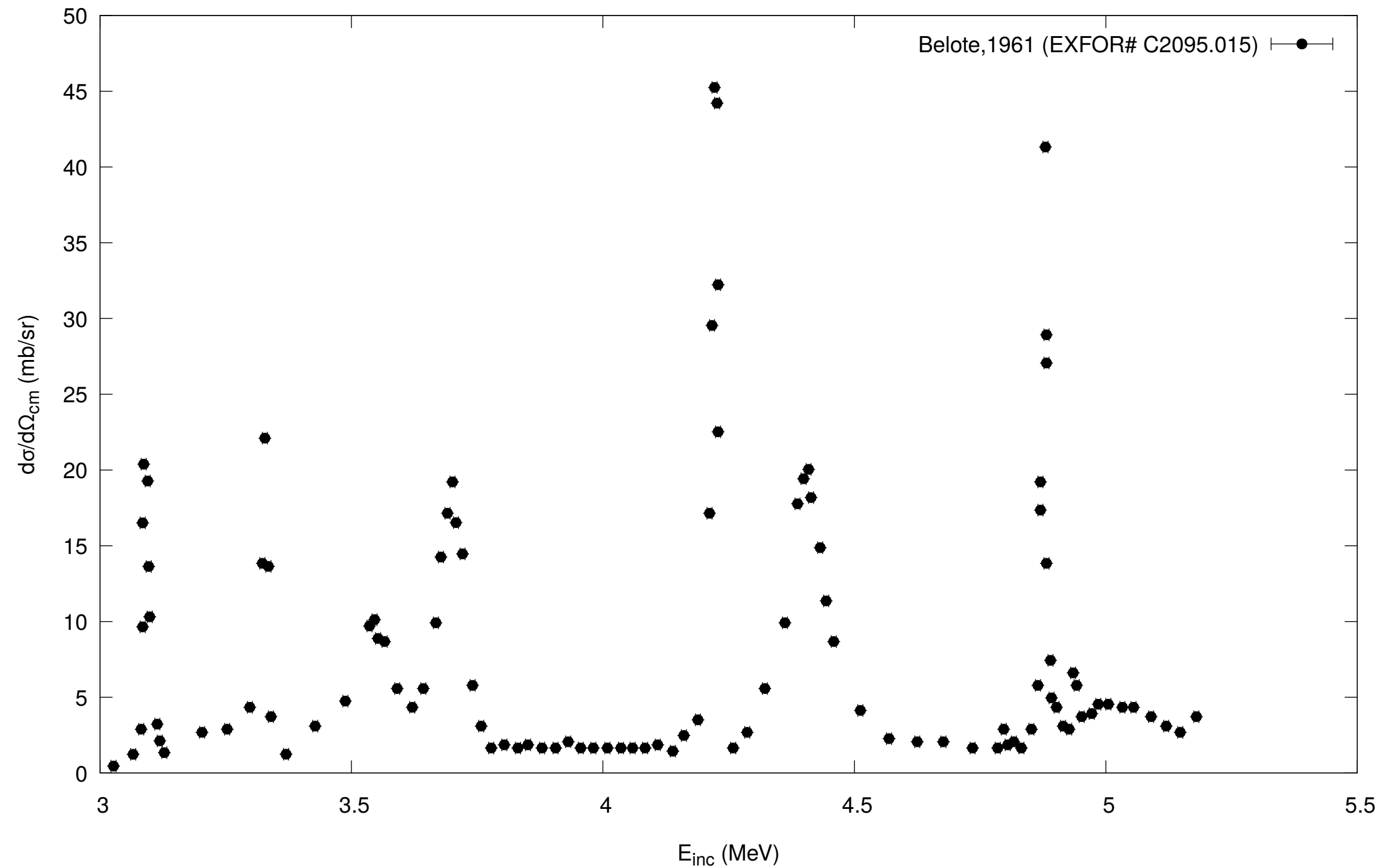
^{28}\text{Si}(p, \text{inl})^{28}\text{Si}, \theta_{\text{lab}} = 165^\circ
