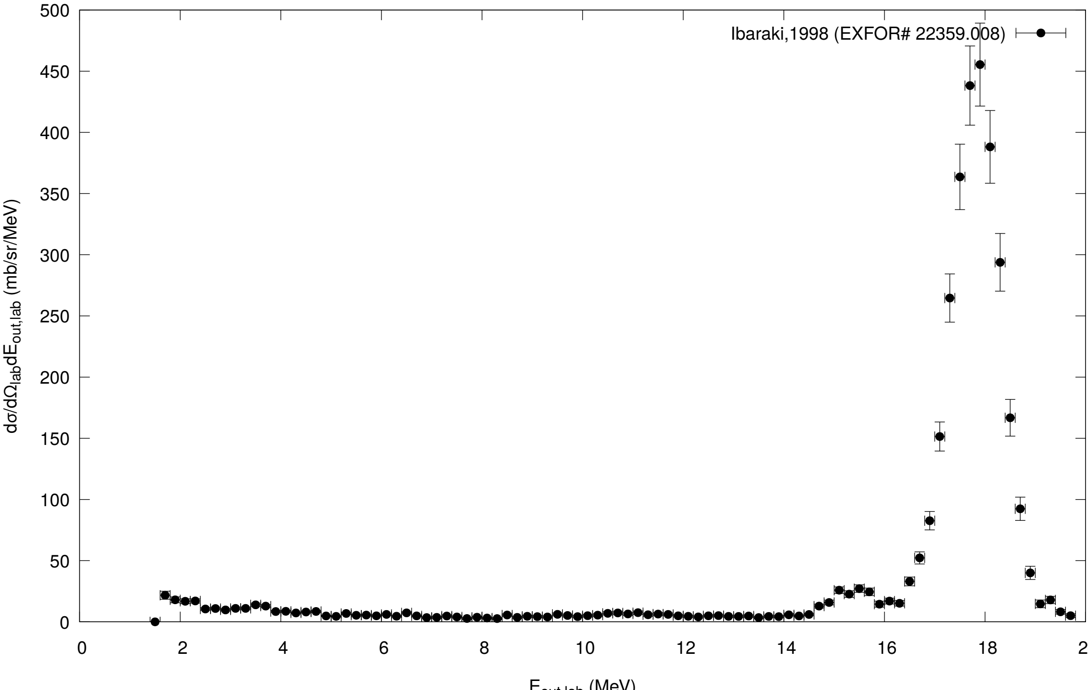
^9\text{Be}(n,n+x), E_{\text{inc}}=18 \text{ MeV}, \theta_{\text{lab}}=20 \text{ deg}
