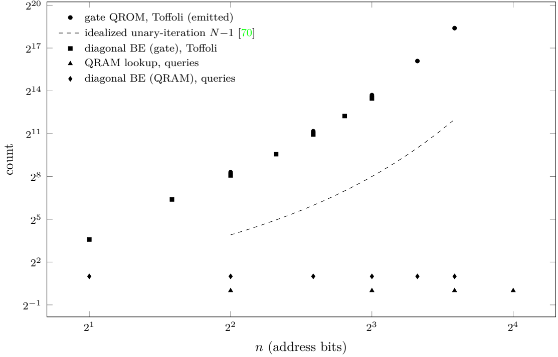
Figure 11: QRAM as a first-class resource, measured. Flat marks are query counts (independent of n ); steep marks are gate-synthesized realizations of the same data access; the dashed line is the idealized unary-iteration QROM model. The vertical separation—one query against 10^4 – 10^5 Toffoli, and the 84\times gap between the idealized model and the emitted network at n=12 —is the quantitative content of the access-model abstraction.
