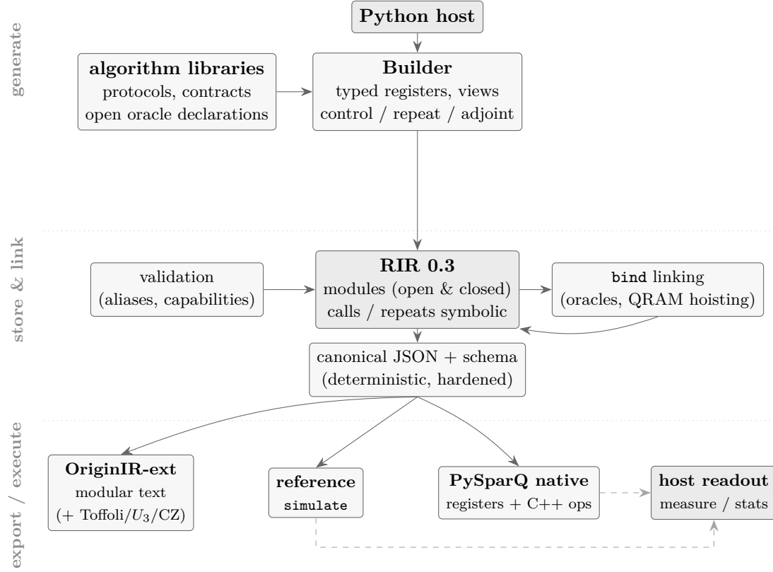
Figure 4: pyqecclang architecture. Programs are generated by the embedded builder and algorithm libraries, stored as RIR (open oracle slots included), optionally linked by bind , serialized to canonical schema-validated JSON, and only then exported or executed. Native backends are imported lazily at execution entry; the core has no backend dependency. Readout is a host-side plan, not an IR construct.
