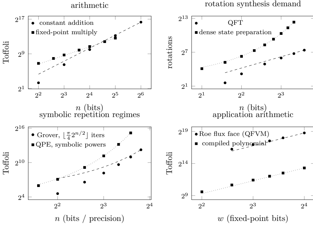
Figure 10: Measured resource scaling of the strict-gate-set estimator (marks) against theoretical reference slopes (dashed/dotted), log-log with base-2 axes. All series come from the JSON artifacts of tools/build_resource_estimates.py ; fitted slopes and R^2 values are collected in Table 11. The Grover and QPE panels are estimated without expanding the symbolic Repeat counts.
