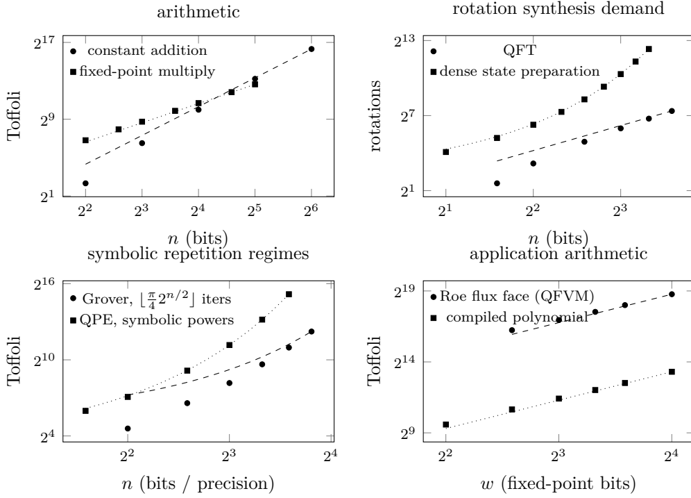
Figure 9: Measured resource scaling of the strict-gate-set estimator (marks) against theoretical reference slopes (dashed/dotted), log-log with base-2 axes. All series come from the JSON artifacts of tools/build_resource_estimates.py ; fitted slopes and R^2 values are collected in Table 13. The Grover and QPE panels are estimated without expanding the symbolic Repeat counts.
