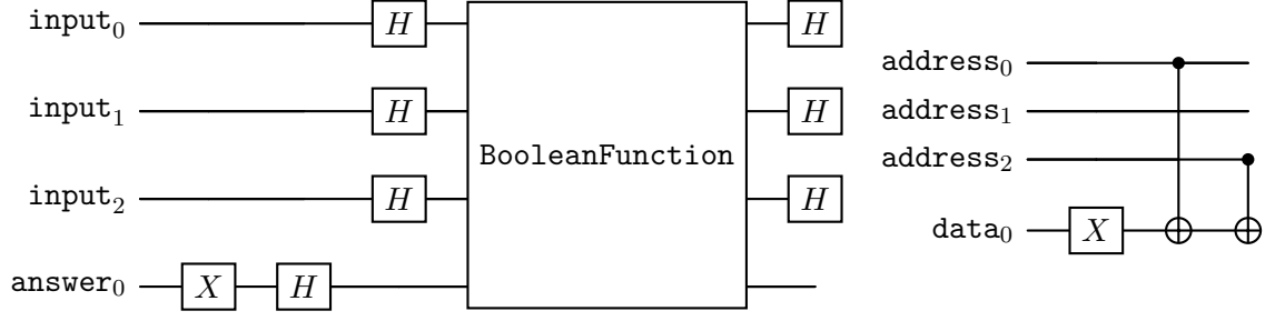
Figure 5: The bound Bernstein–Vazirani program of Listing 3, drawn by the quantikz export. Left: the algorithm as generated—three input wires, one answer wire, and the oracle as a single box named by its slot ( BooleanFunction ); this is the whole program, with no oracle internals materialized. Right: the realization that bind attached for this run (the affine oracle with secret 5, bias 1): an X on the data wire and two XOR controls from address bits 0 and 2. The two circuits are modules of one program; the algorithm circuit is unchanged whichever realization closes the slot.
