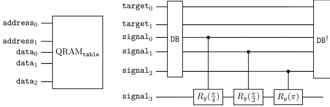
Figure 6: Two QRAM idioms, drawn by the quantikz export. Left: a bare Load—one instruction on the address and data registers, |a\rangle|d\rangle \mapsto |a\rangle|d \oplus M[a]\rangle , with the table itself a runtime resource. Right: the diagonal block-encoding of an angle table ( D_{jj} = \alpha \cos(s d_j/2) , here s = \pi/4 , \alpha = 1 ): query the angle database, apply one controlled R_y per angle bit onto the flag wire, unquery. The same ladder realizes the coefficient angle databases of the input-model matrix (Table 10); the database box is again a slot, bindable to a gate truth table or a QRAM resource.
