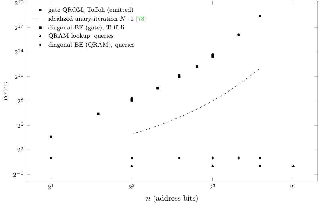
Figure 10: QRAM as a first-class resource, measured. Flat marks are query counts (independent of n ); steep marks are gate-synthesized realizations of the same data access; the dashed line is the idealized unary-iteration QROM model. The vertical separation—one query against 10^4 – 10^5 Toffoli, and the 84\times gap between the idealized model and the emitted network at n=12 —is the quantitative content of the access-model abstraction.
