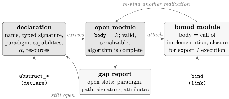
Figure 4: The oracle lifecycle. Declarations create open modules that are carried inside otherwise-complete programs; gap analysis reports what remains open; the binding pass attaches implementations (partially and repeatedly, with compatibility checks and QRAM resource hoisting) until the program is closed for export or execution.
