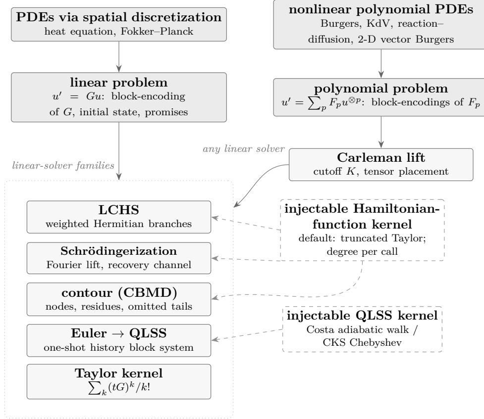
Figure 7: The ODE/PDE solver territory of pyqecclang. Linear problems feed four evolution- and system-oriented families (LCHS, Schrödingerization, contour decomposition, Taylor kernels) plus the QLSS-based history-system family; nonlinear polynomial problems lift through Carleman into the same linear-solver position. Dashed boxes mark injectable protocols : the kernel realizing e^{-iHt} subroutines and the linear-system kernel are swappable arguments, as are the spatial discretizers connecting the PDE layer to the problem layer.
