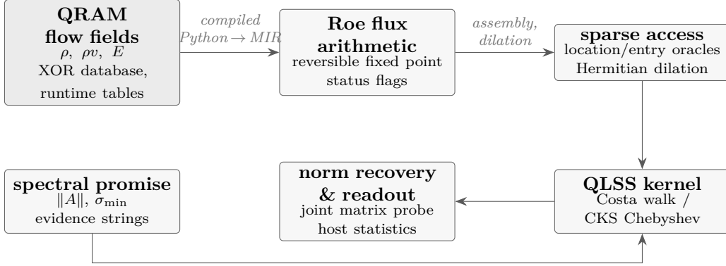
Figure 8: The QFVM pipeline for the one-dimensional compressible Euler equations. Flow fields are served coherently from a QRAM; Roe flux formulas written as pure Python are compiled to reversible arithmetic; the implicit-step operator is exposed as a sparse-access oracle pair; and the linear solve is an injected QLSS kernel operating under an explicit spectral promise. Its fixed-point physics is certified against an independent fixed-point semantics in the verification matrix of Section 9.
