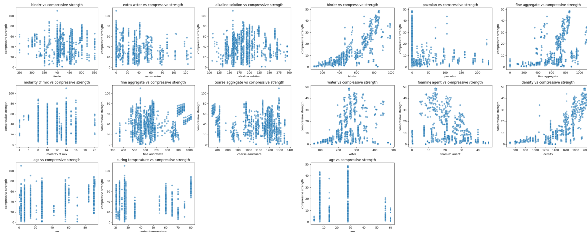
Figure 3: Scatter plots of key features against compressive strength for the geopolymer and lightweight datasets, used to identify non-linear relationships and potential outliers.
