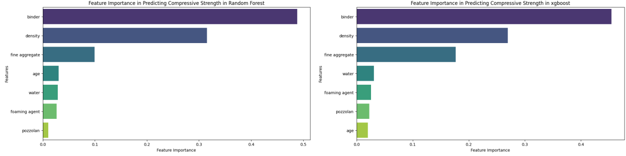
Figure 7: Feature importance plots for Random Forest and XGBoost on the lightweight dataset (individual analysis).
