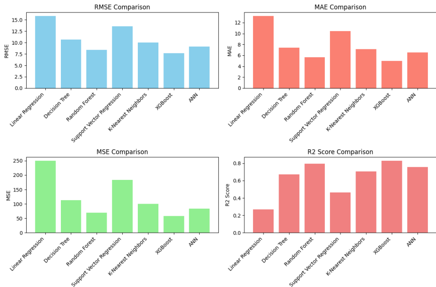
Figure 4: Bar graph comparing performance metrics of different ML models on the geopolymer dataset (individual analysis).
