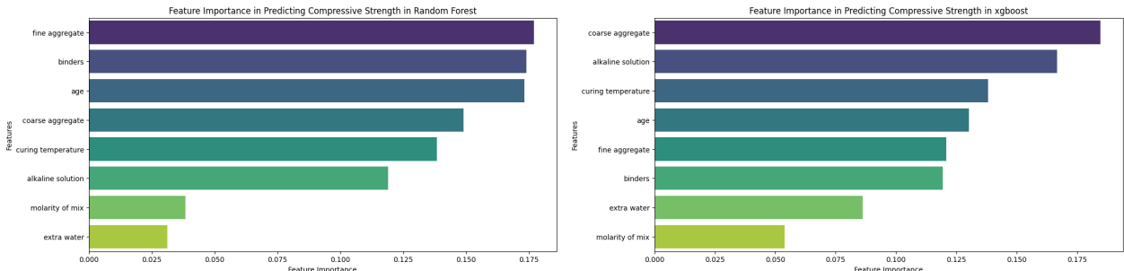
Figure 5: Feature importance plots for Random Forest and XGBoost on the geopolymer dataset (individual analysis).
