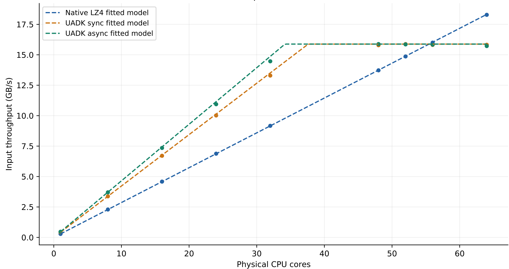
8 KiB window: measured points and fitted saturation model
