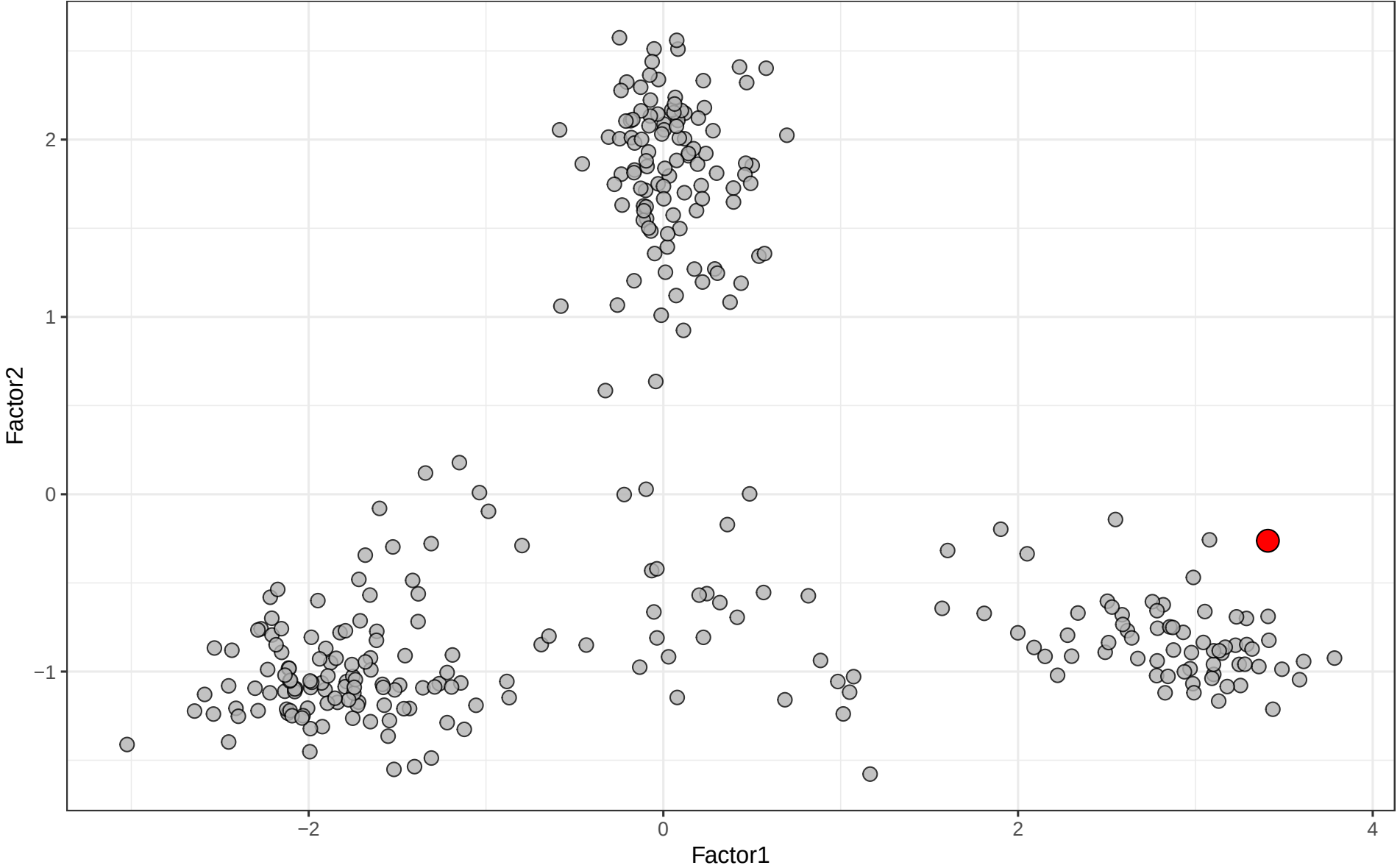
SRR10720231 | Factor1 vs Factor2
