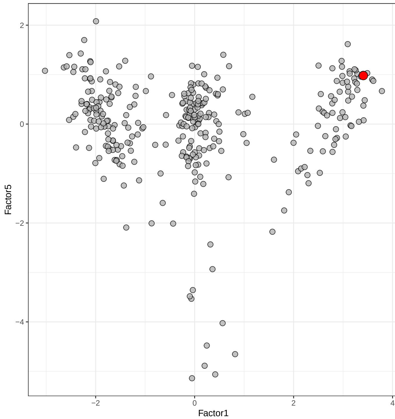
SRR10720231 | Factor1 vs Factor5
