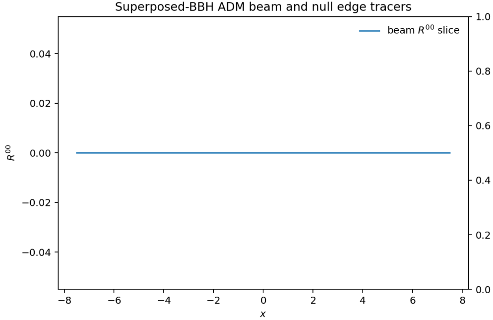
Figure 5: ADM beam slice on the superposed binary black-hole background with null particle trajectories initialized on the edge of the beam cone.
