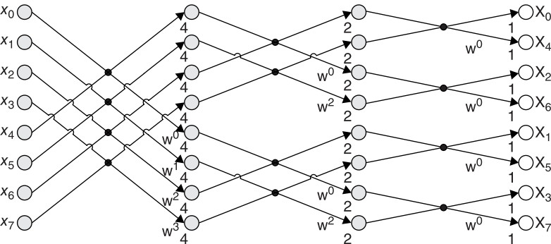
(b) FFT structure
