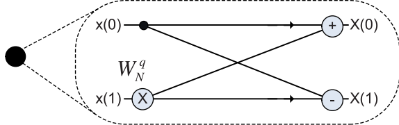
(a) FFT element
