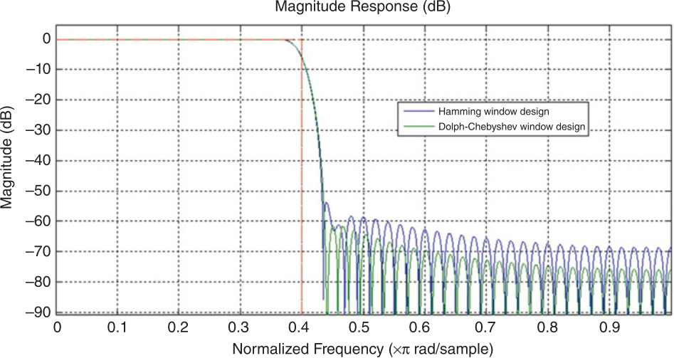
(a) 100-tap response
