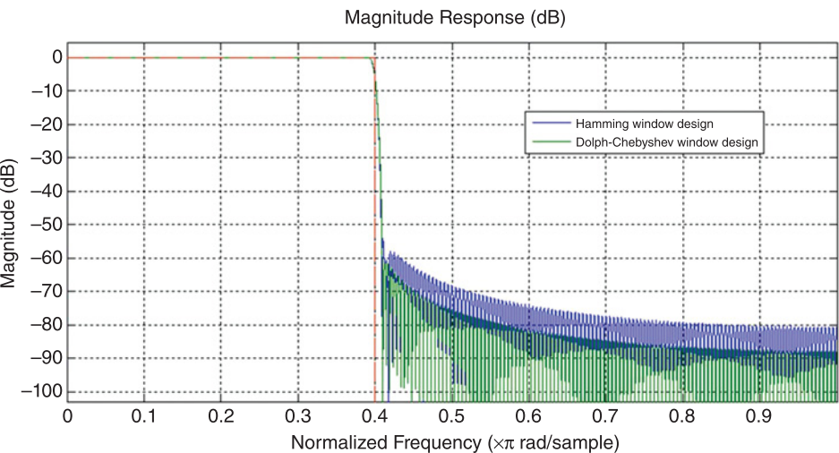
(b) 400-tap response
