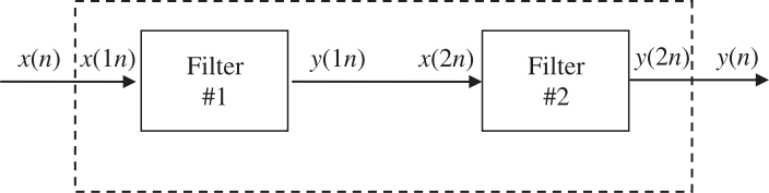
(a) Cascade FIR filter
