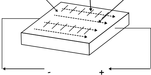
a) Movement of electrons without magnetic field
