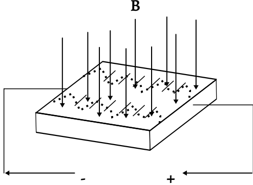
b) Movement of electrons with magnetic field
