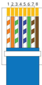
RJ45 Pinout T-568B
