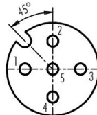
Female insert M12
