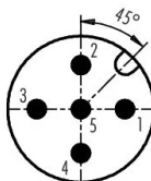
Male insert M12
