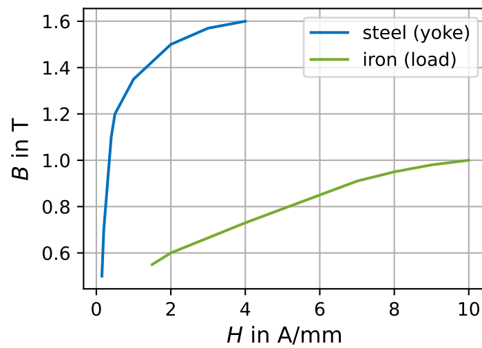
Figure 2: Magnetization curves for the yoke (steel) and the load (iron).
