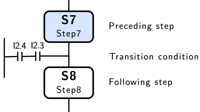
Transition programmed in LAD
