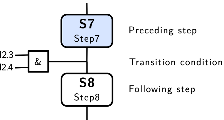
Transition programmed in FBD
