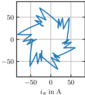
nonlinear machine model
