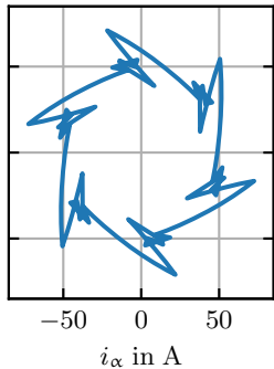
Nonlinear machine model
