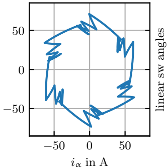
linear machine model
