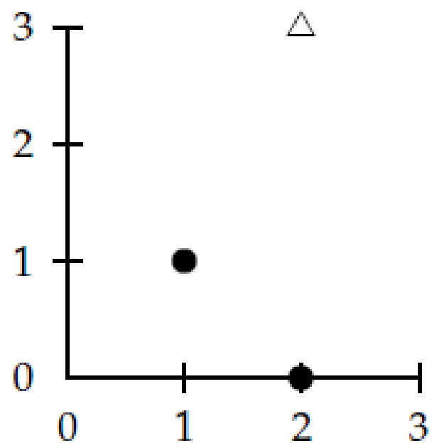
► Figure 15.4 A tiny 3 data point training set for an SVM.
