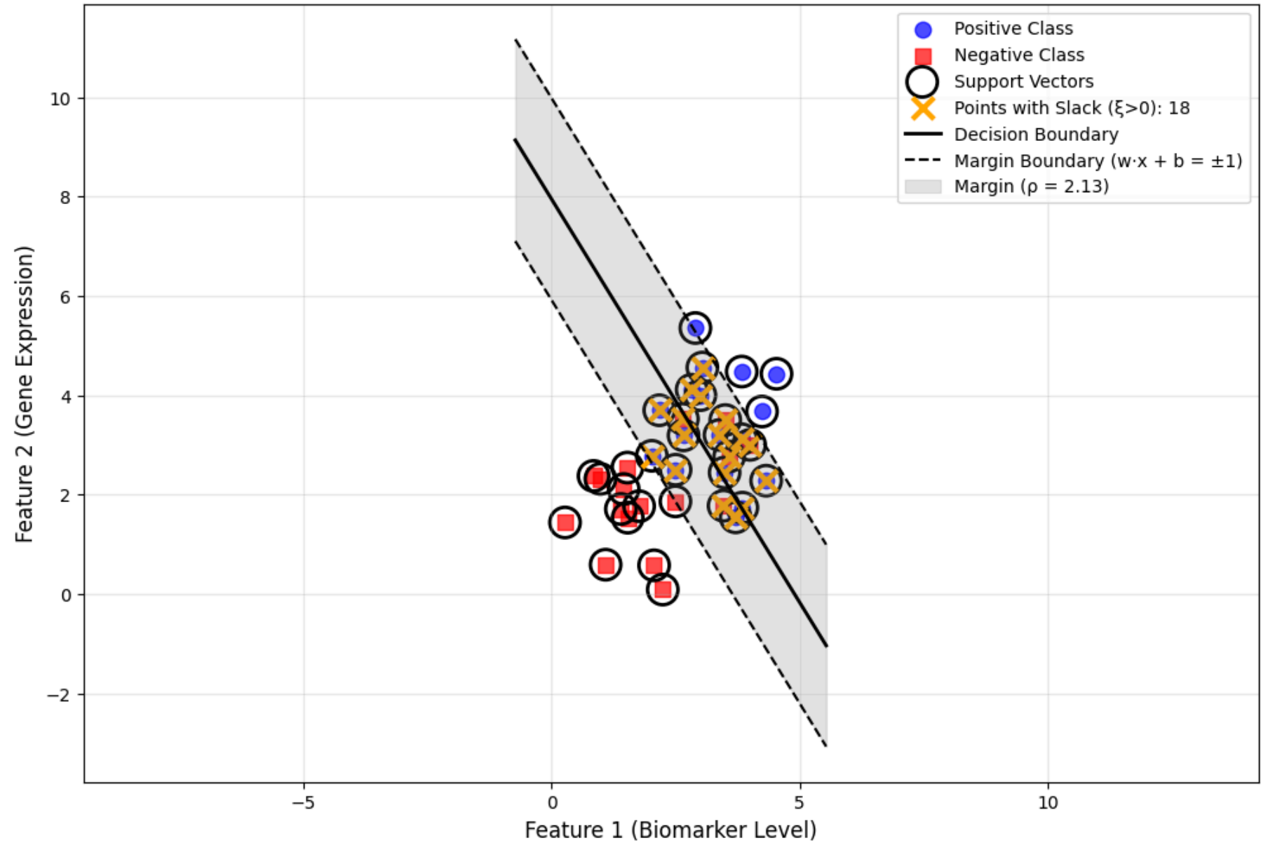
Hard-Margin SVM on Non-separable Data C=1000000.0, Support Vectors=34, Margin=2.129
