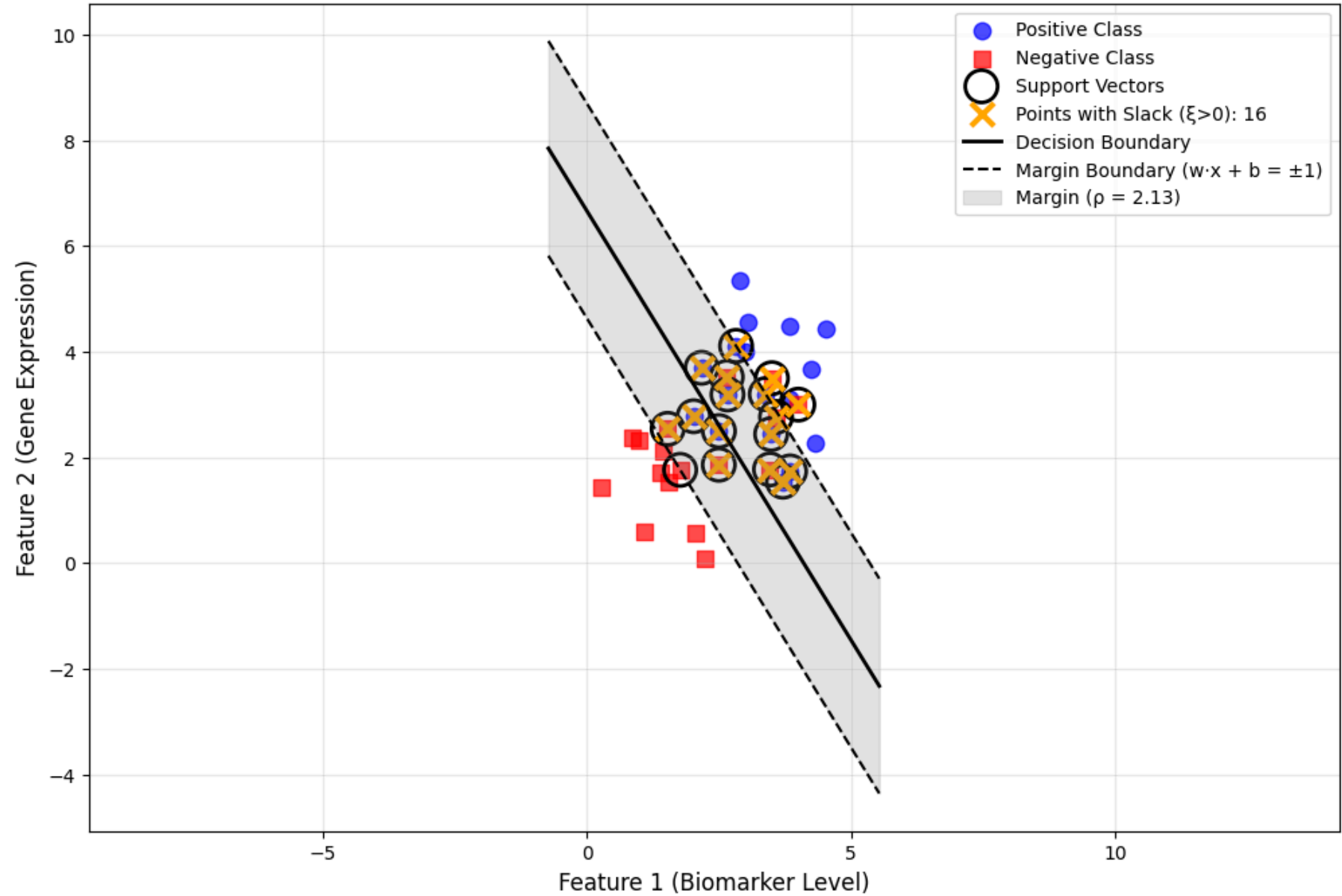
Medical Diagnosis with Soft-Margin SVM (C=100.0) C=100.0, Support Vectors=17, Margin=2.129
