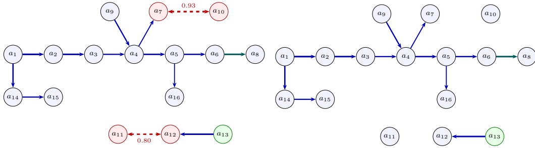
(a) Incoherent (base). Two EXCLUSIVE conflicts (dashed): a_7 \leftrightarrow a_{10} is unresolved ; a_{11} \leftrightarrow a_{12} is a concession the holding a_{13} (green) resolves. mm = 0.607 , \log Z = -9.64 . (b) Coherent . The identical support structure with both conflict edges removed; a_{10} and a_7 are no longer suppressed. mm = 0.620 , \log Z = -8.25 , lp = 1.00 .
