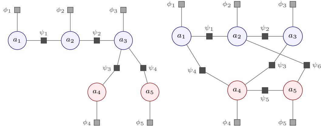
(a) Response A. Five unaries and four pairwise factors.
