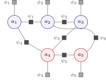
(b) The MRF it induces: one \psi_r per edge (black), one \phi_i per prior (grey).
