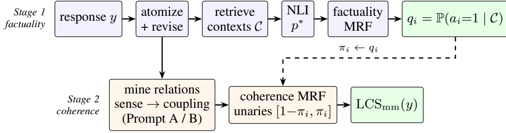
Figure 1: The two-stage pipeline. Stage 1 (§3) is FactReasoner (Marinescu et al., 2025): it grounds each atom against retrieved evidence and returns a posterior marginal q_i . Stage 2 (§4) builds a second MRF over the atoms alone and adds one pairwise factor per mined atom–atom relation; the mined relation already carries its Level-1 coupling, so no separate compile step intervenes. The dashed arrow is the only coupling between the stages, and carries the composition \pi_i \leftarrow q_i into the \phi_i = [1 - \pi_i, \pi_i] of Def. 1. Atomization is shared, so the response is decomposed once and both stages score the same claim set; setting \pi_i \equiv \frac{1}{2} instead recovers a pure coherence score that consults no external evidence (Rem. 3).
