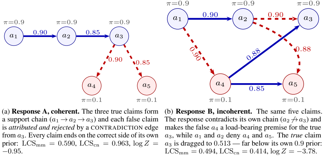
Figure 2: Relation graphs for the five-claim worked pair (§10). Blue nodes are claims true of the world ( \pi_i = 0.9 ), red nodes false ( \pi_i = 0.1 ); the same five claims appear in both panels. Solid blue: ENTAILMENT; dashed red: CONTRADICTION. Line width grows with the relation weight p . The panels differ only in how the response arranges the claims, which is the whole of what coherence measures — no per-claim factuality check can separate them.
