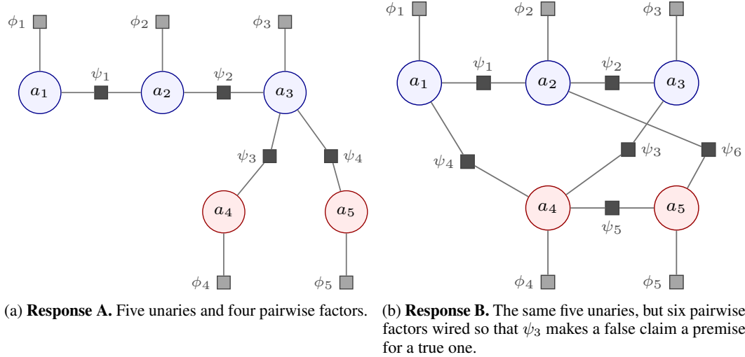
Figure 3: The coherence MRF of Eq. 2 for the two responses, as an explicit factor graph. Circles are the binary claim variables; grey squares the unary factors \phi_i = [1 - \pi_i, \pi_i] that carry the priors; black squares the pairwise factors \psi_{\tau_r, p_r} of Table 2, one per mined relation. The priors enter only through the \phi_i : the claim-level potentials are identical across the two panels, and every difference in score comes from the \psi_r — their number, their endpoints, and their couplings.
