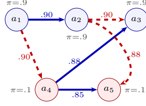
(a) The relation graph: three ENTAILMENT (solid blue), three CONTRADICTION (dashed red); width grows with p .
