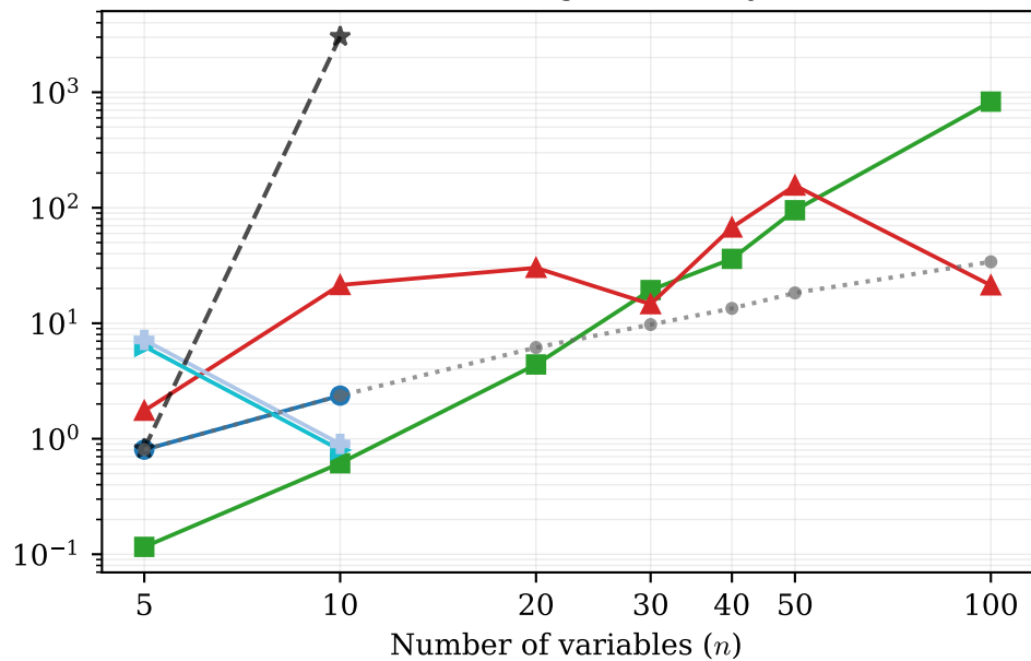
Run time (algorithm only)
