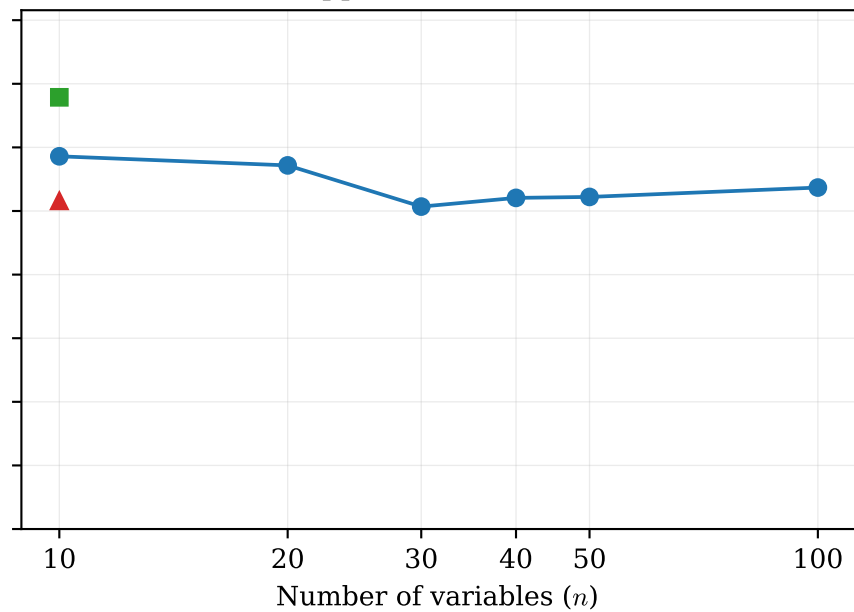
Upper bound error
