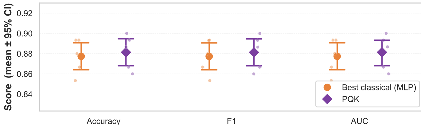
A. Performance: PQK vs best classical (MLP) [hvg] (n=5 splits)
