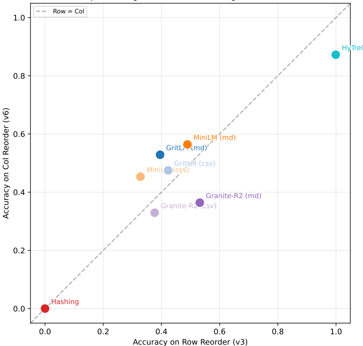
Row vs Column Perturbation Sensitivity (hi-pos/hi-neg, default window, avg over datasets)
