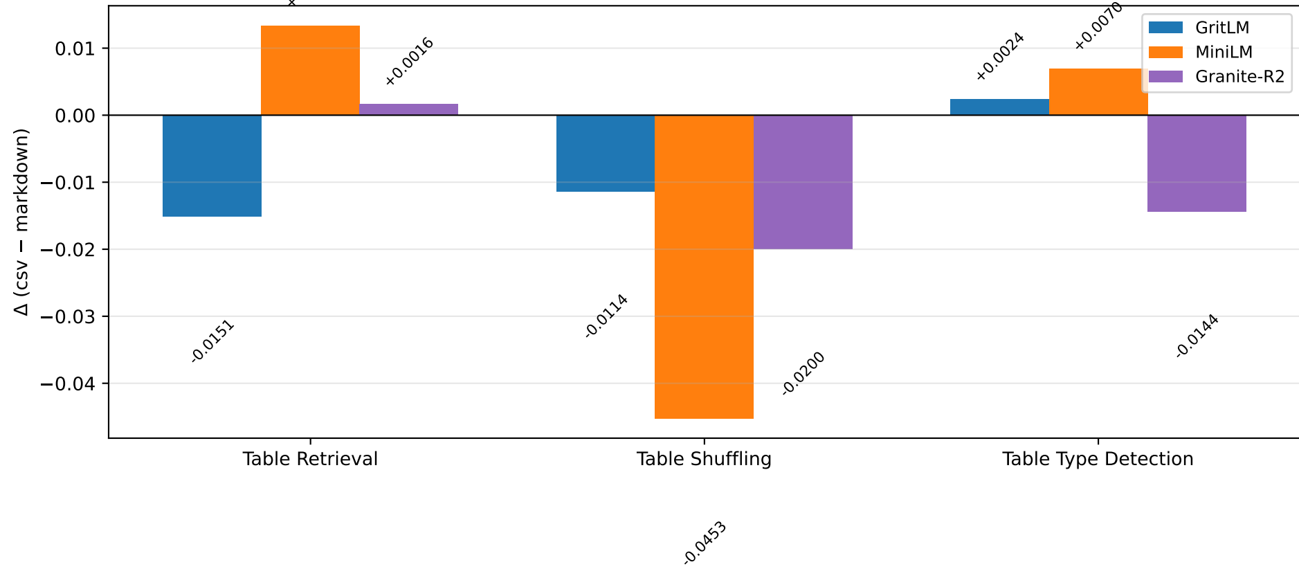
Serialization Impact: CSV vs Markdown Across Tasks
