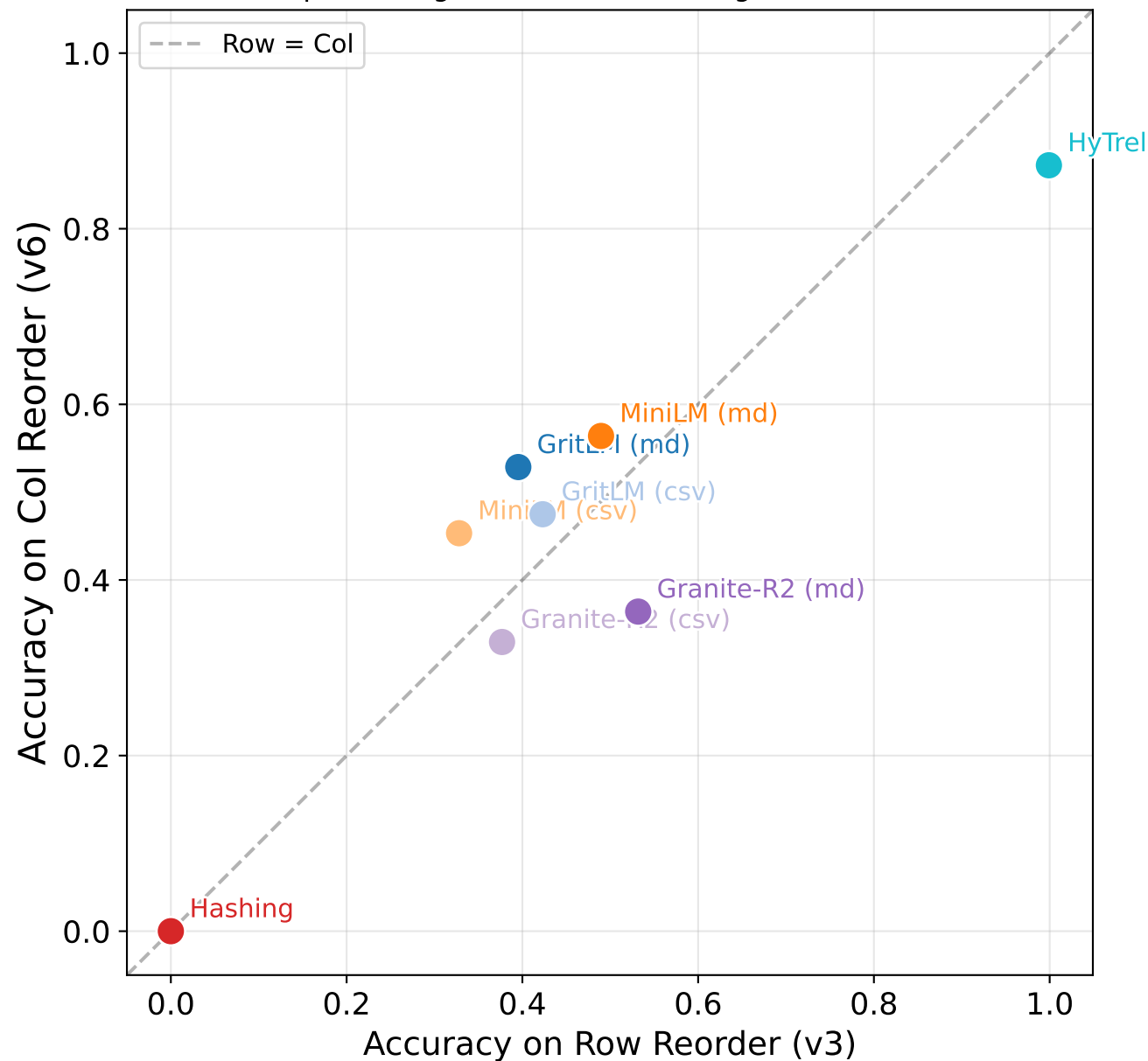
Row vs Column Perturbation Sensitivity (hi-pos/hi-neg, default window, avg over datasets)
