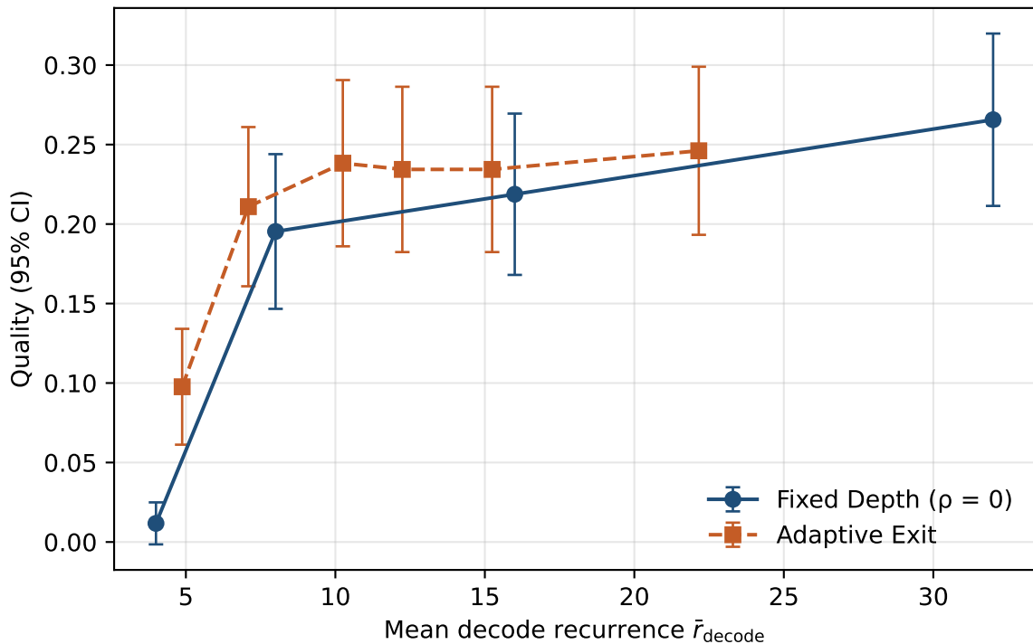
gsm8k: quality vs mean recurrence
