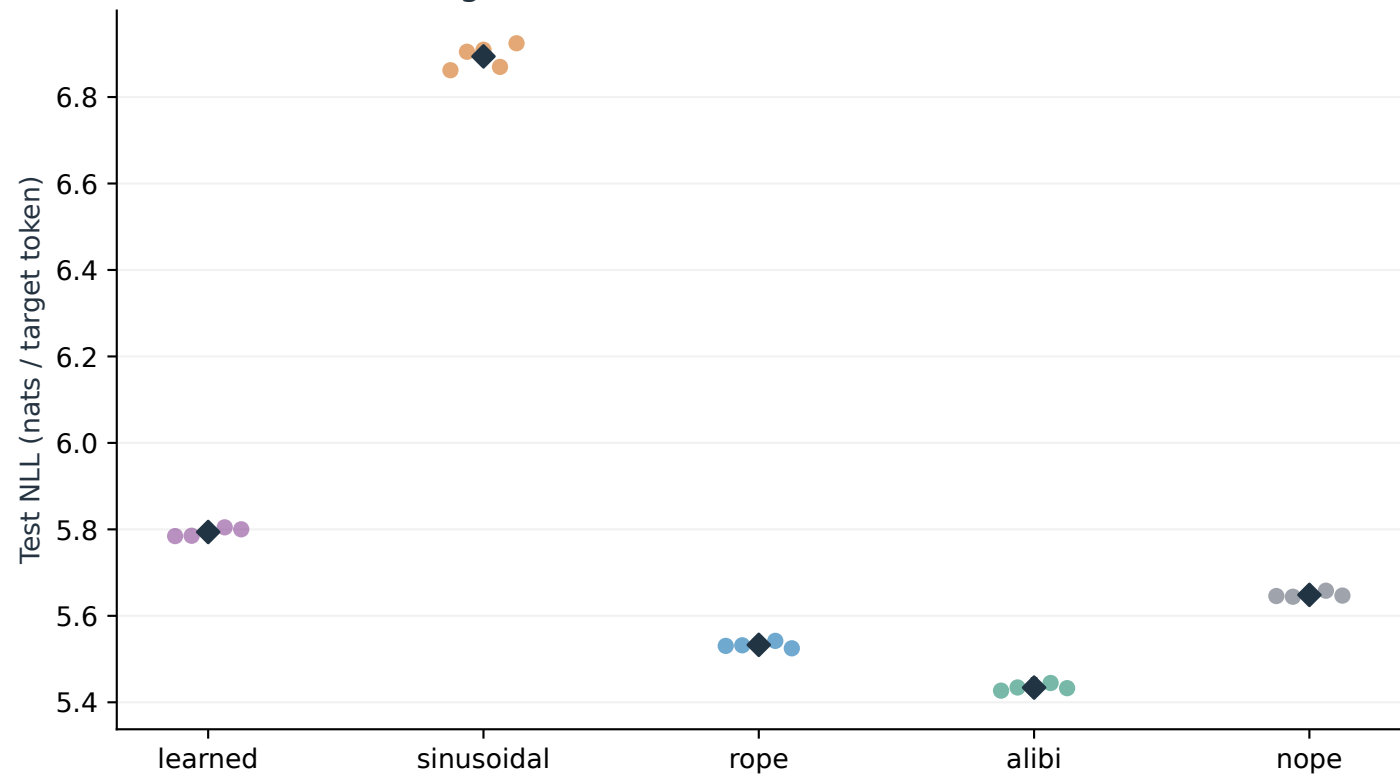
Figure 5 · Final models at context 512
