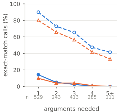
(c) Each argument costs
