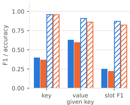
(b) Where grounding fails
