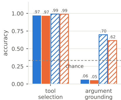
(a) Selection vs. grounding
