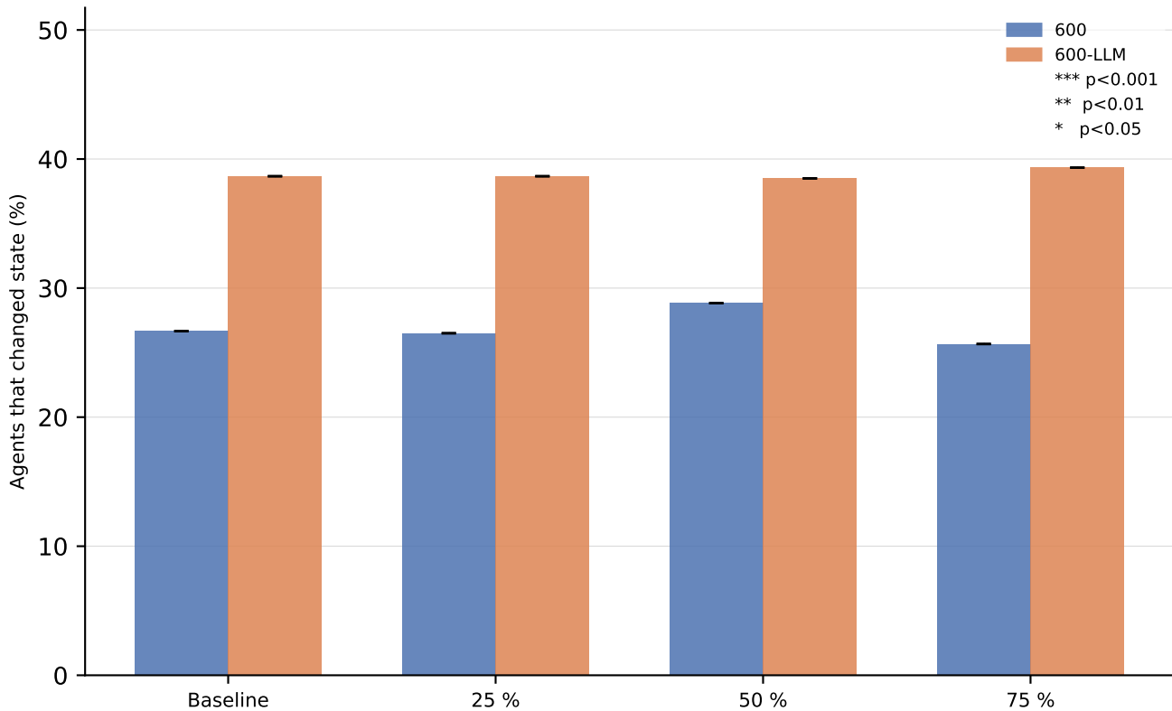
Agents that changed state (%) — all threads (credulous)
