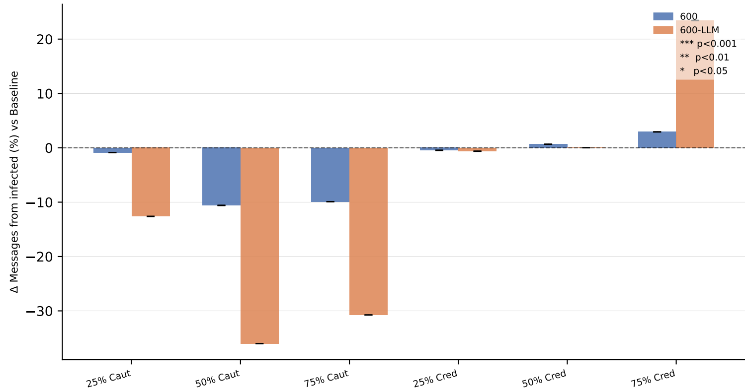
\Delta vs Baseline — Messages from infected (%) — all threads
