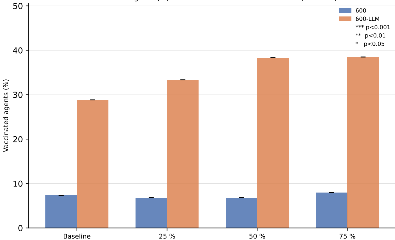
Vaccinated agents (%) — thread 524949443607412737 (cautious)
